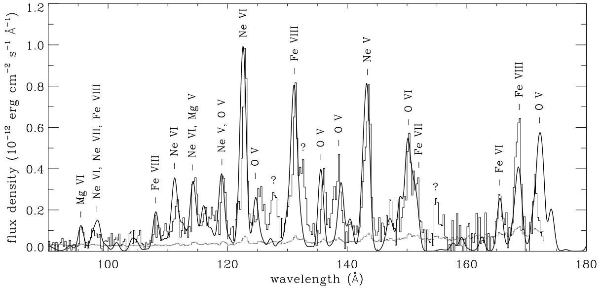
Fig. 1. Mean EUVE spectrum of OY Car. The spectrum is shown by the black histogram, the error by the grey histogram, the scattering model spectrum by the thick line. Line identifications are based on the model.
